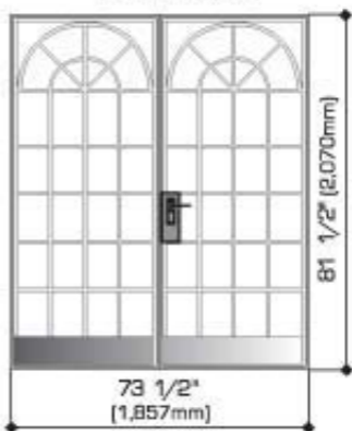
Steel Arched Door Double Leaf
