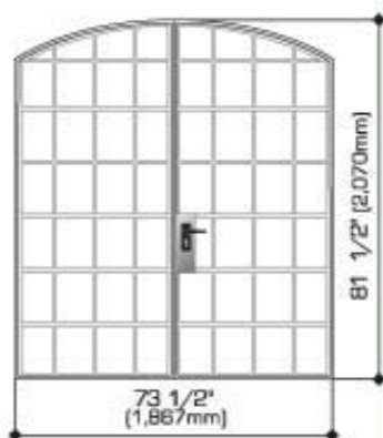
Steel Arched Double Leaf Door
